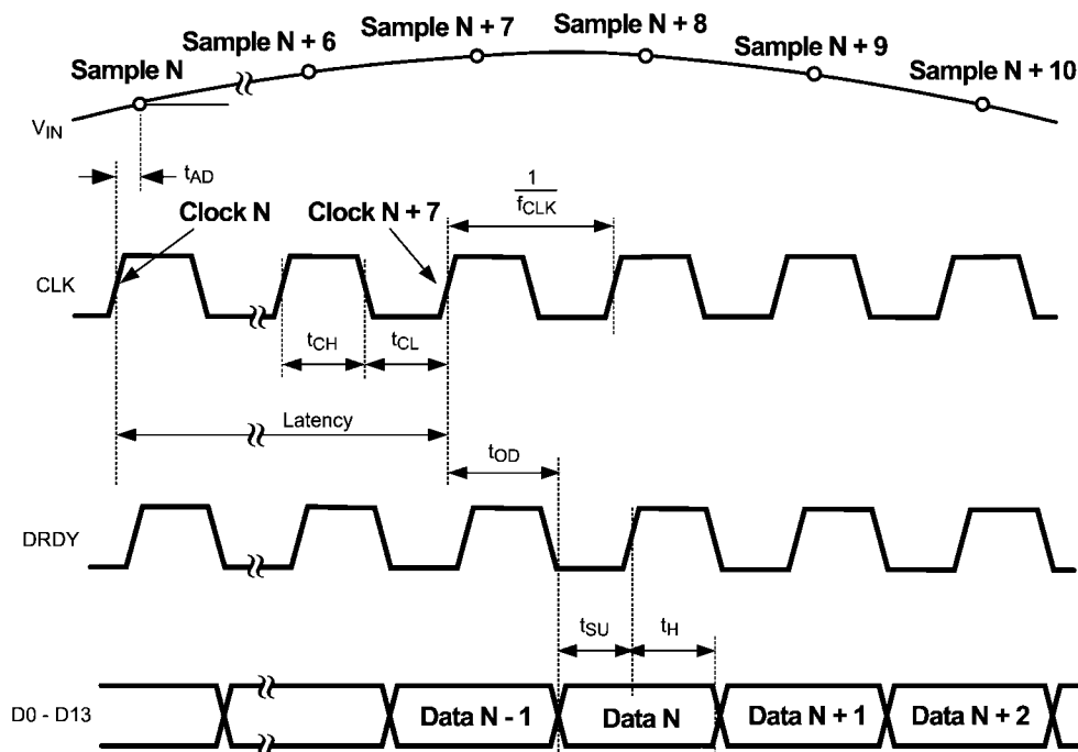
FIGURE 1. Output Timing
